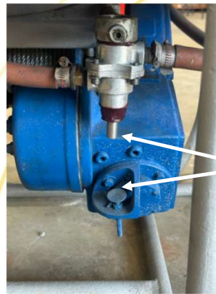
Overload Switch Alignment
